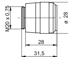
ZLENS-OCS.22MM 11224617
