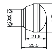
ZLENS-OCS.40MM 11224640
