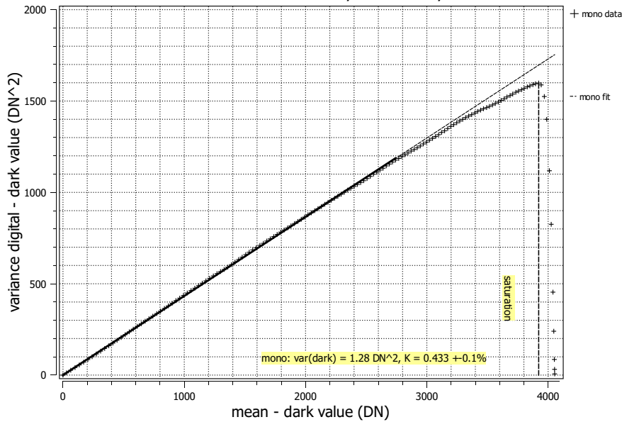
Photon transfer mACC300150, 533 nm, 01.06.2023
