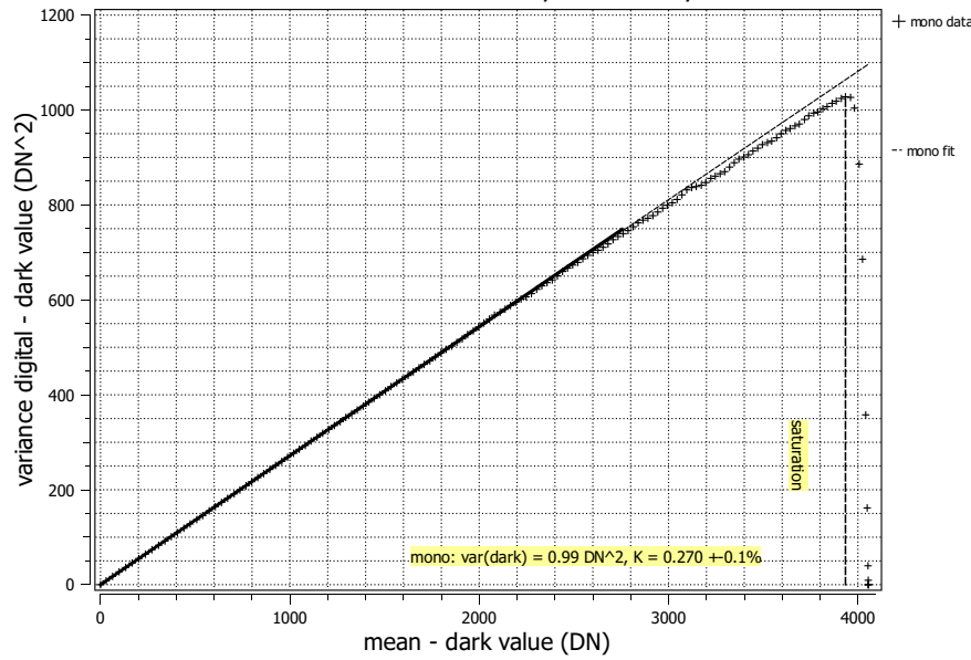
Photon transfer mACC300244, 533 nm, 10.10.2023
