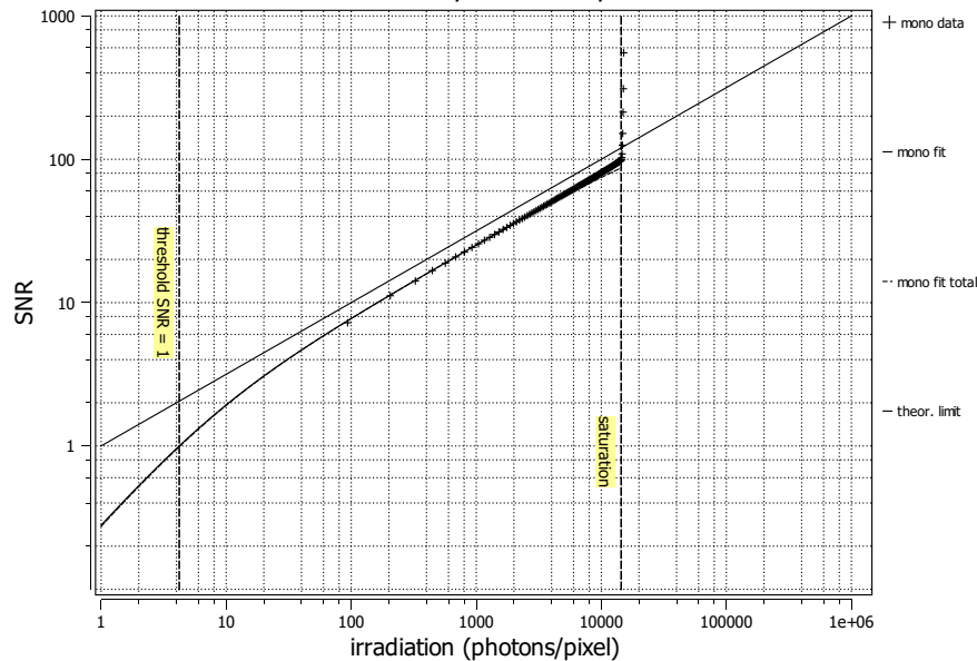
SNR mACC300238, 533 nm, 12.09.2023
