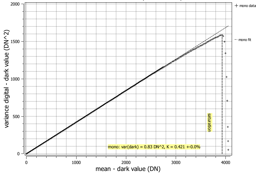
Photon transfer mACC300238, 533 nm, 12.09.2023
