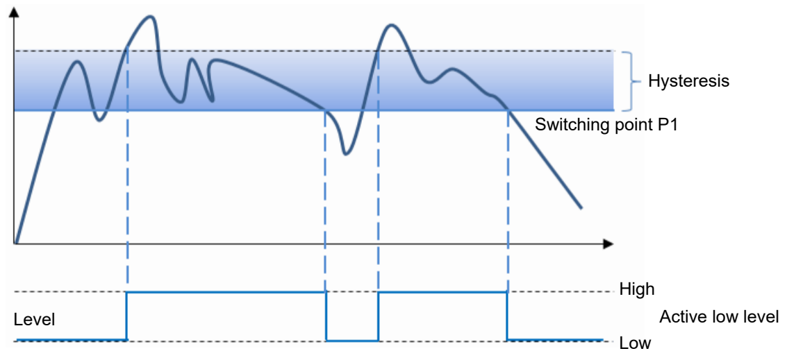
III. 11: Behavior of the switching output in point mode (positive hysteresis)
