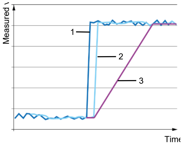
III. 4: Moving Average filter
