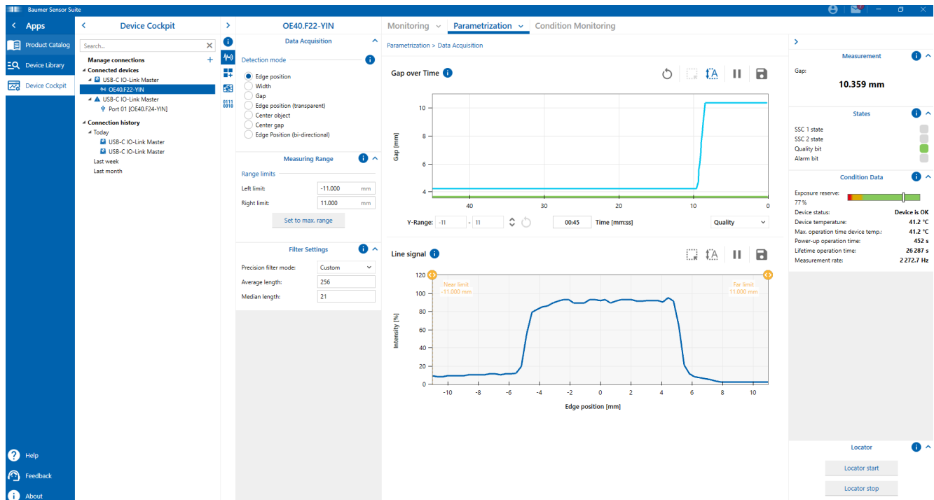
III. 15: Representation of exposure reserve (with BSS as an example)
