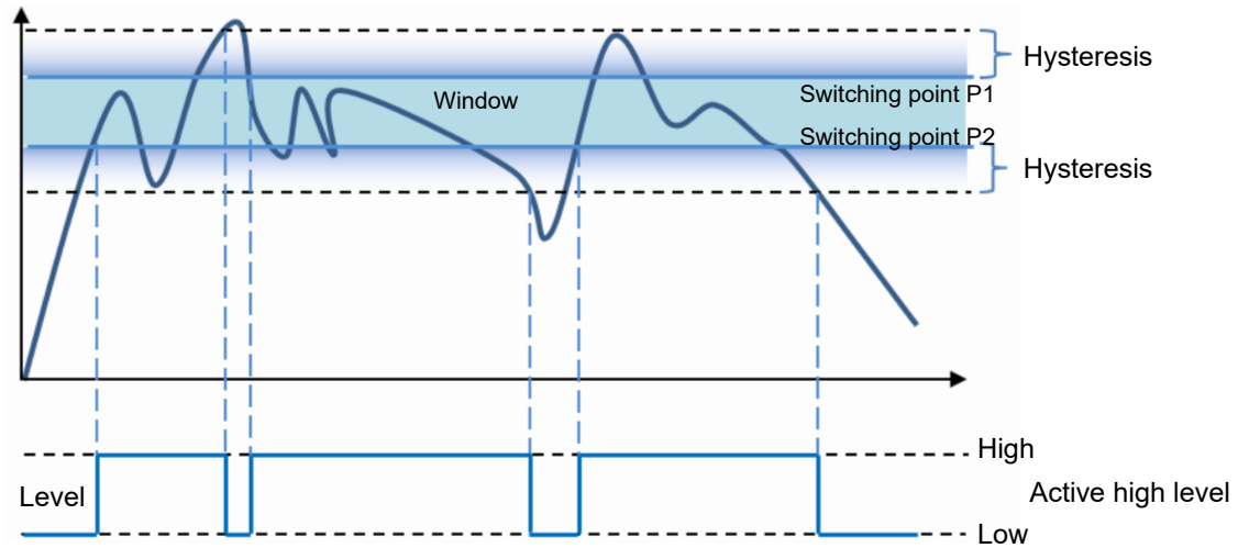
III. 12: Behavior of the switching output in window mode (positive hysteresis)
