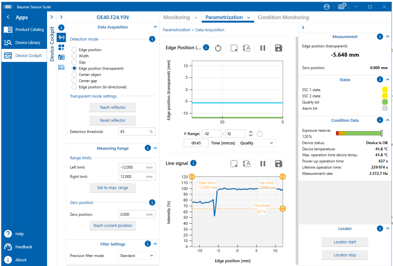
III. 2: Edge position (transparent) settings on the example of BSS
