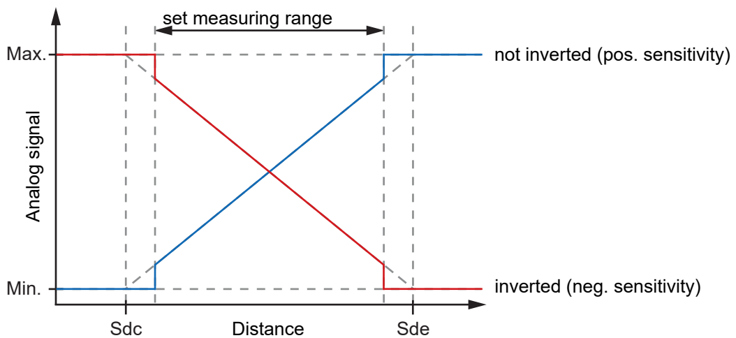
Ill. 13: Analog output - Inverted
