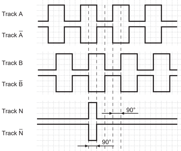
NI-Output signals
