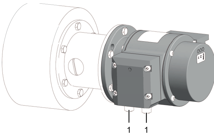
Abb. 7: Anschlüsse HOG980.M
