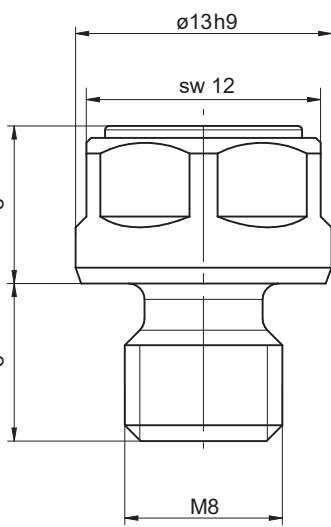
Threaded screw M8 x 8, \phi 13 x 8
